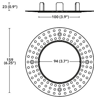
DMR50 Downlight Trimless Adapter Round
