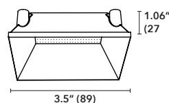
DTSAW50 Downlight Trim Square Adjustable IP44 (Solite Lens)
