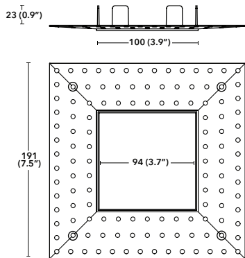
DMS50 Downlight Trimless Adapter Square
